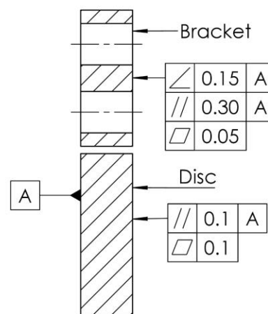
Mounting specification
