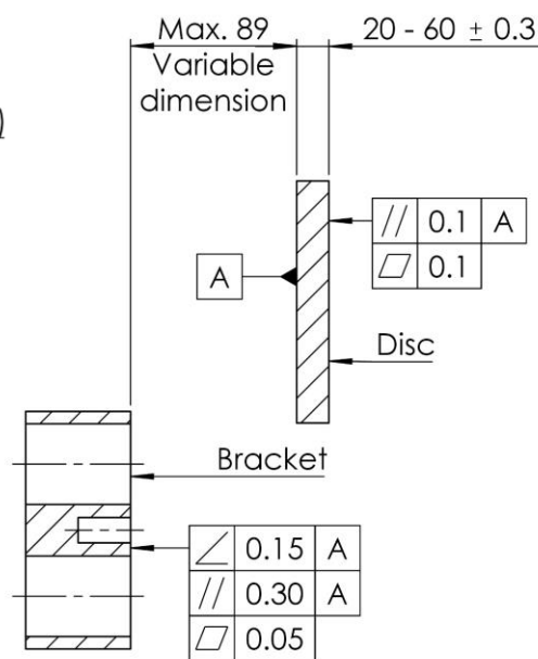
Mounting specification
